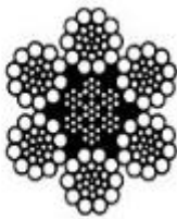
6X25 Filler Wire with IWRC 6x26 Warrington Seale with IWRC
